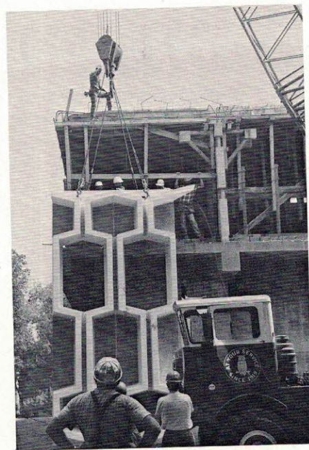
Six ton element hoisted into place.
